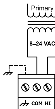
AC Powered
